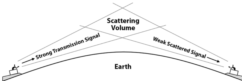
Figure 3. Troposcatter Communication Signal Propagation
